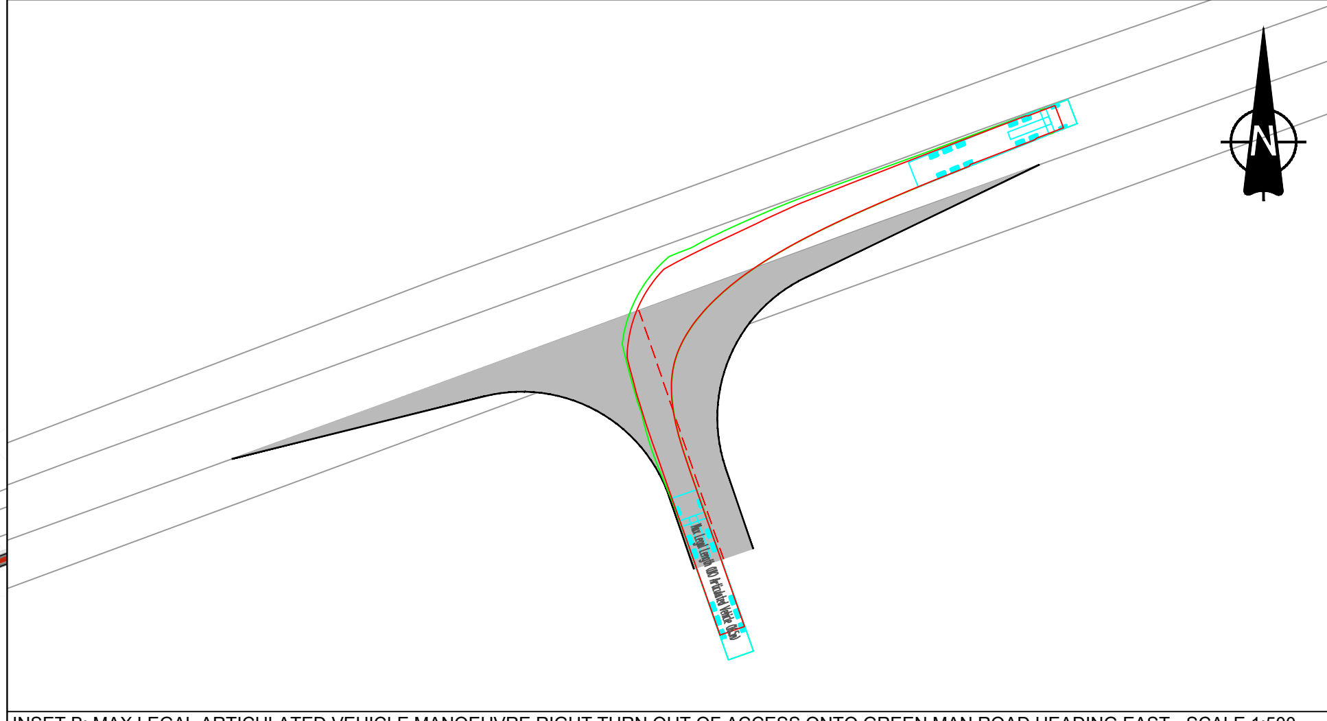
INSET B: MAX LEGAL ARTICULATED VEHICLE MANOEUVRE RIGHT TURN OUT OF ACCESS ONTO GREEN MAN ROAD HEADING EAST - SCALE 1:500
