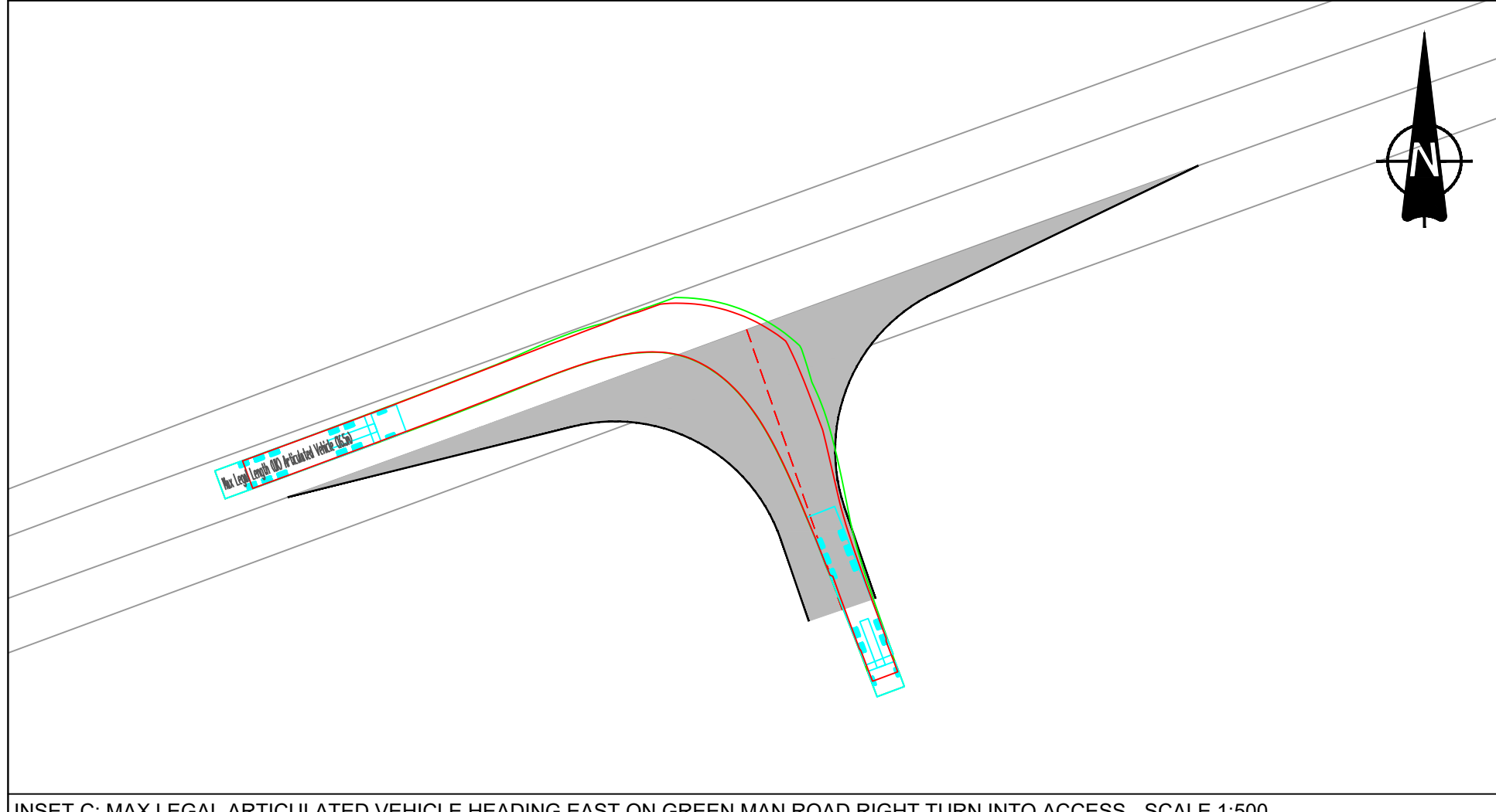
INSET C: MAX LEGAL ARTICULATED VEHICLE HEADING EAST ON GREEN MAN ROAD RIGHT TURN INTO ACCESS - SCALE 1:500
