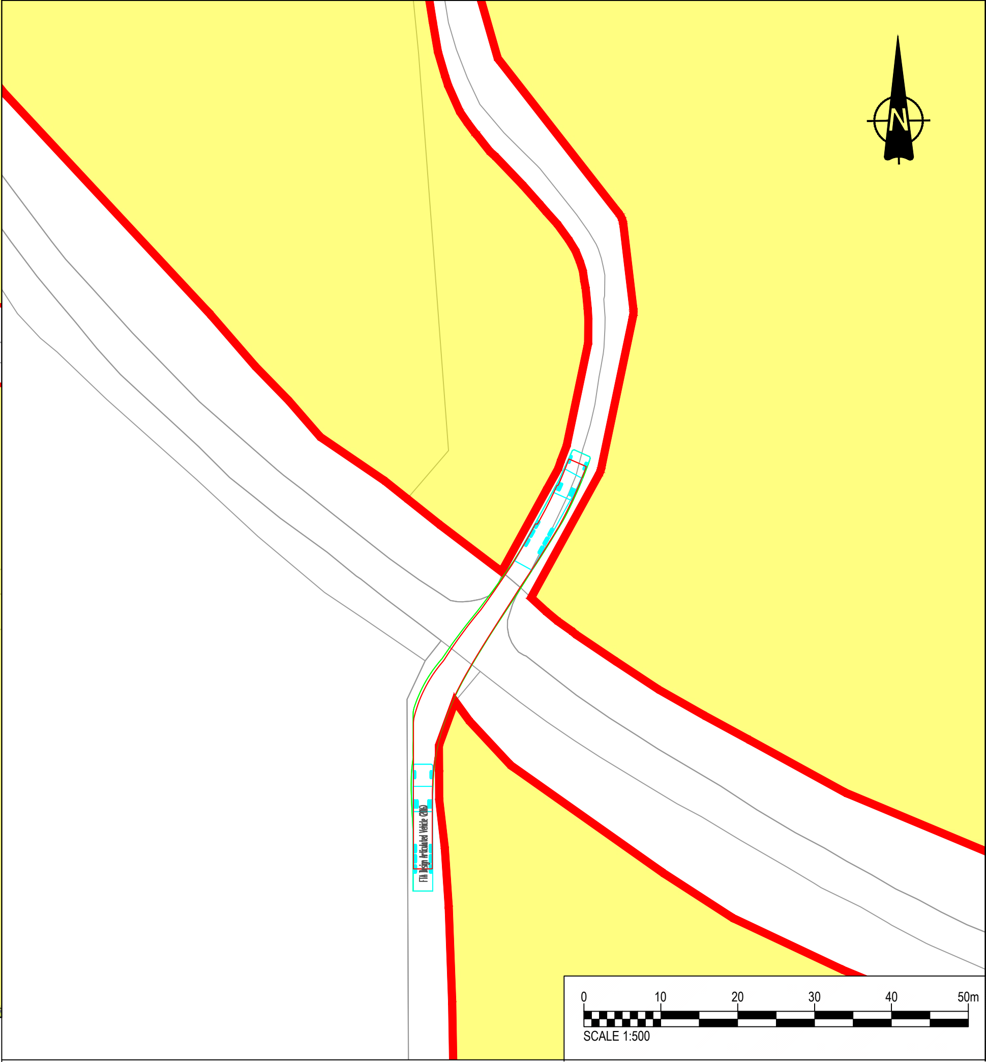
INSET B: ARTICULATED VEHICLE CROSSING STONE LANE HEADING NORTH - SCALE 1:500
