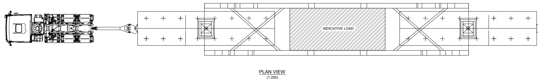
VEHICLE CONFIGURATION - 16-AXLE GIRDER TRAILER (Refer notes)
