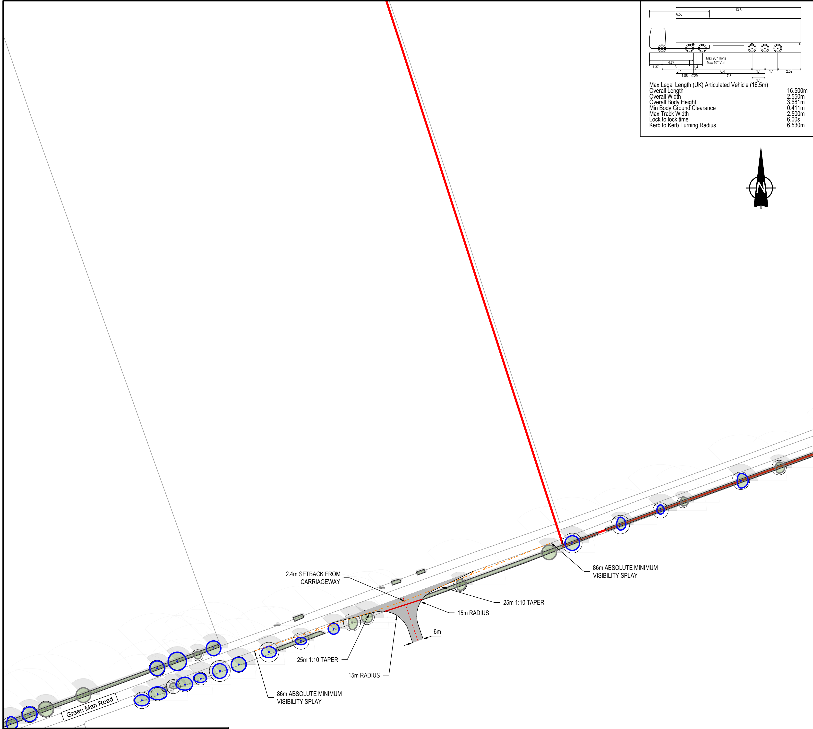
INSET A: MAX LEGAL ARTICULATED VEHICLE MANOEUVRE LEFT TURN OUT OF ACCESS ONTO GREEN MAN ROAD HEADING WEST - SCALE 1:500
