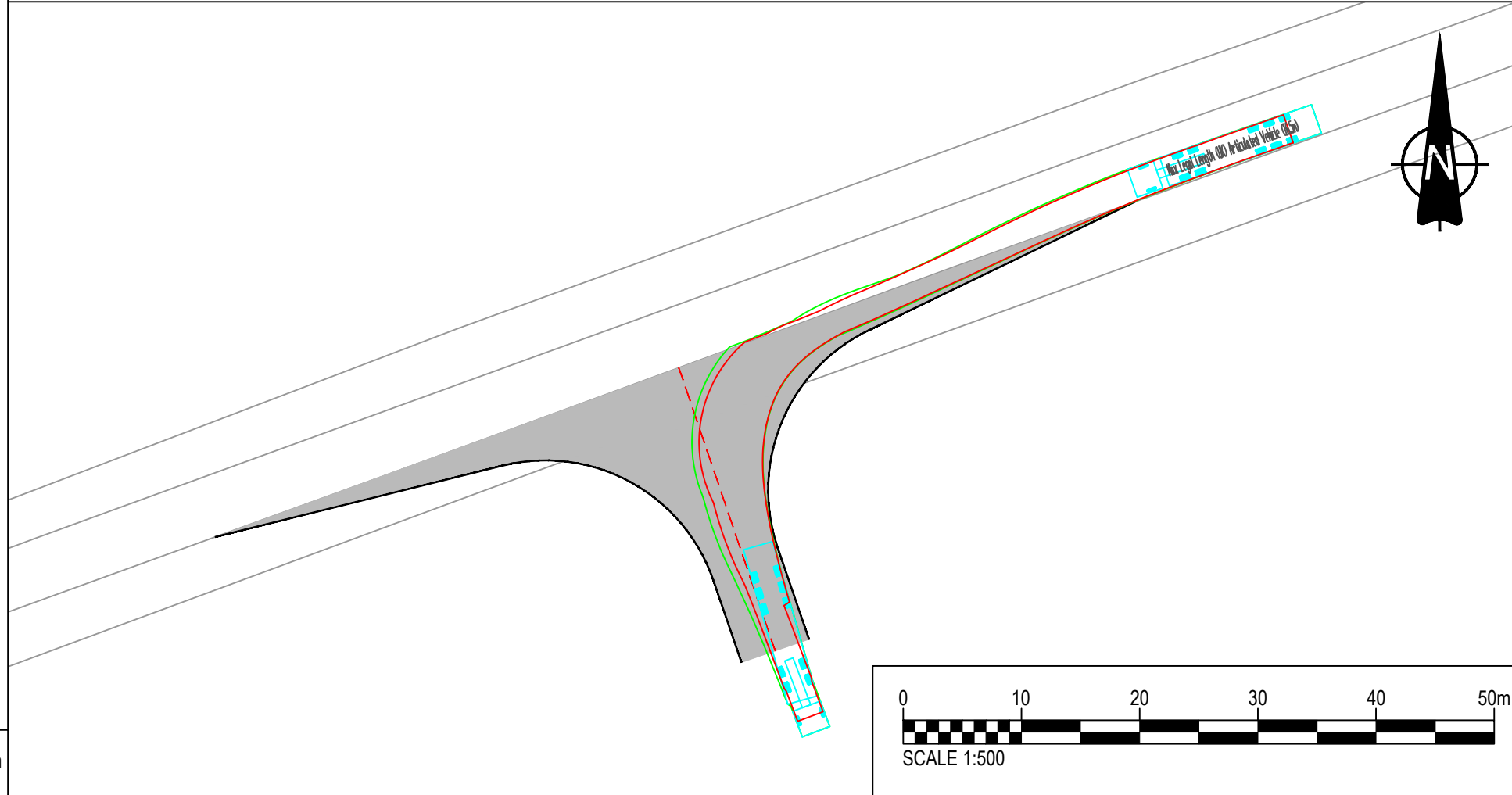
INSET D: MAX LEGAL ARTICULATED VEHICLE HEADING WEST ON GREEN MAN ROAD LEFT TURN INTO ACCESS - SCALE 1:500
