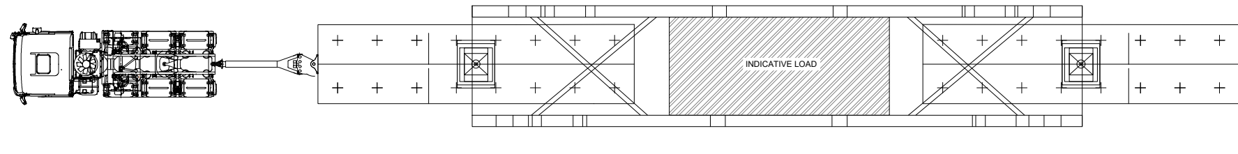
VEHICLE CONFIGURATION - 16-AXLE GIRDER TRAILER (Refer notes)
