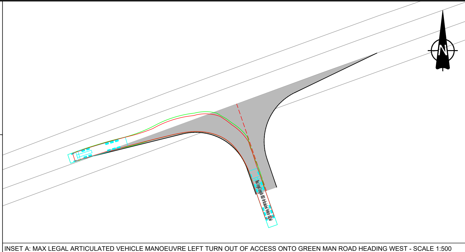
INSET A: MAX LEGAL ARTICULATED VEHICLE MANOEUVRE LEFT TURN OUT OF ACCESS ONTO GREEN MAN ROAD HEADING WEST - SCALE 1:500
