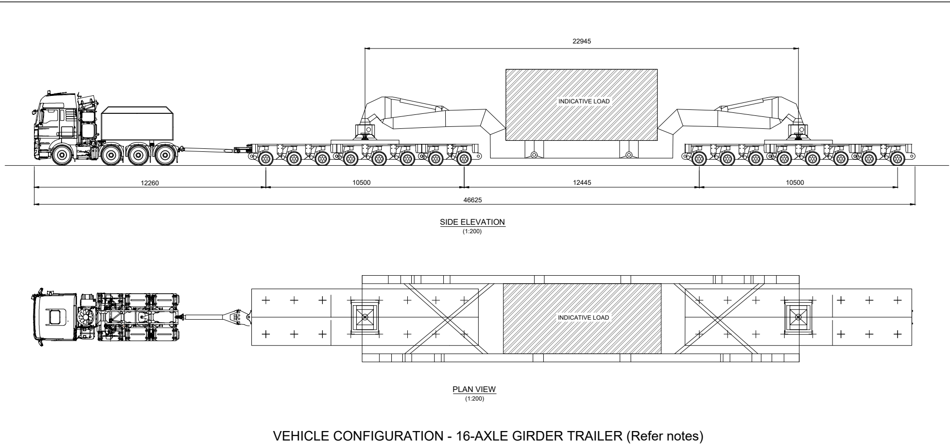
VEHICLE CONFIGURATION - 16-AXLE GIRDER TRAILER (Refer notes)
